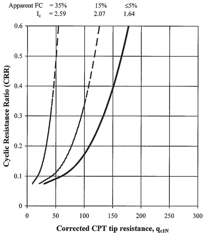
Fig. 11. CPT base curves for various values of soil behaviour index, I_c (corresponding to various apparent fines contents, as indicated).
