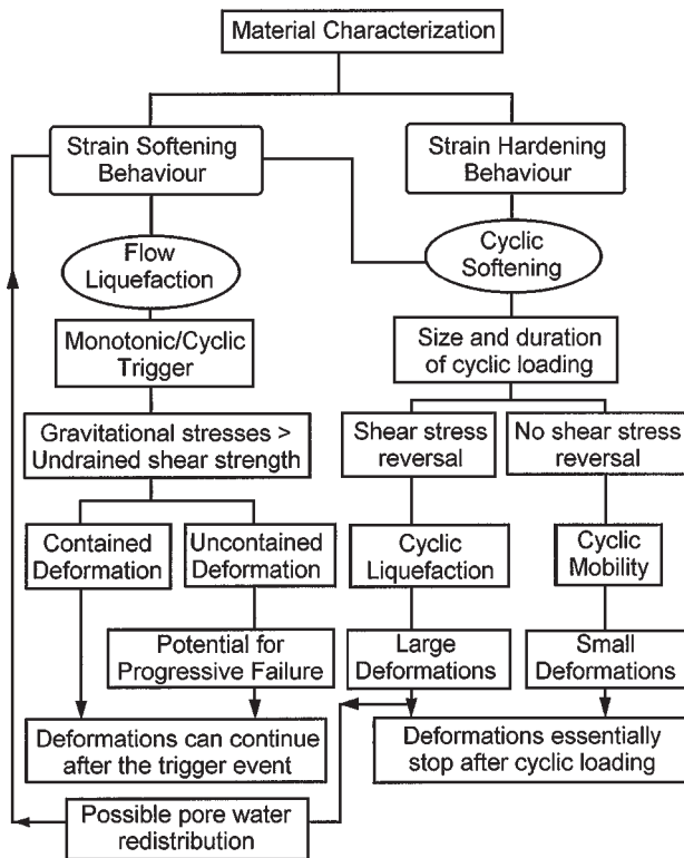
Fig. 3. Suggested flow chart for evaluation of soil liquefaction (after Robertson 1994).
