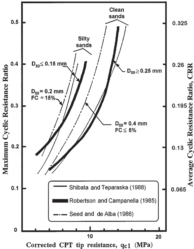
Fig. 5. Comparison between three CPT-based charts for estimating cyclic resistance ratio (CRR) for clean sands (after Ishihara 1993). D_{50} , average grain size; FC, fines content.
