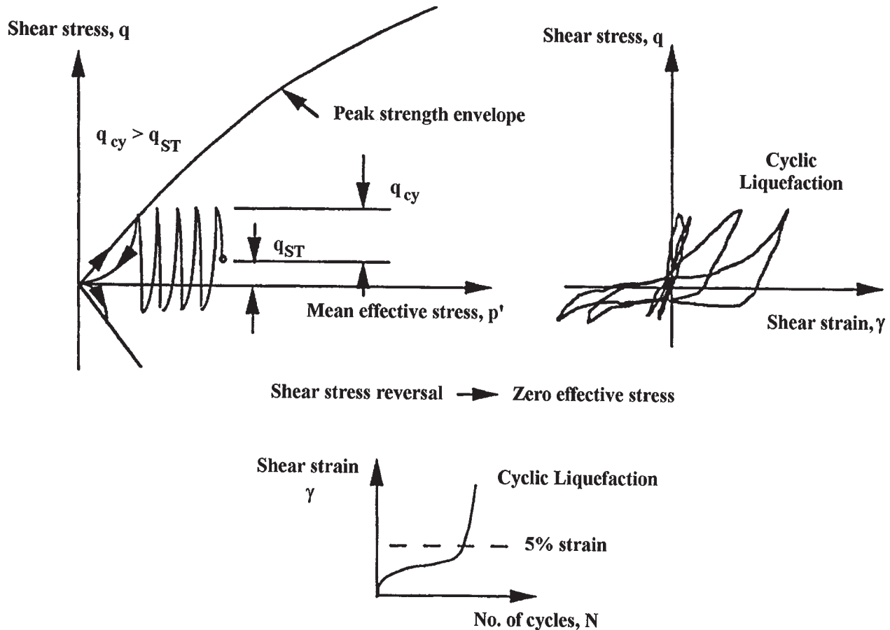
Fig. 2. Schematic of undrained cyclic behaviour of sand illustrating cyclic liquefaction (after Robertson 1994). q_{cy} , cycling shear stress.
