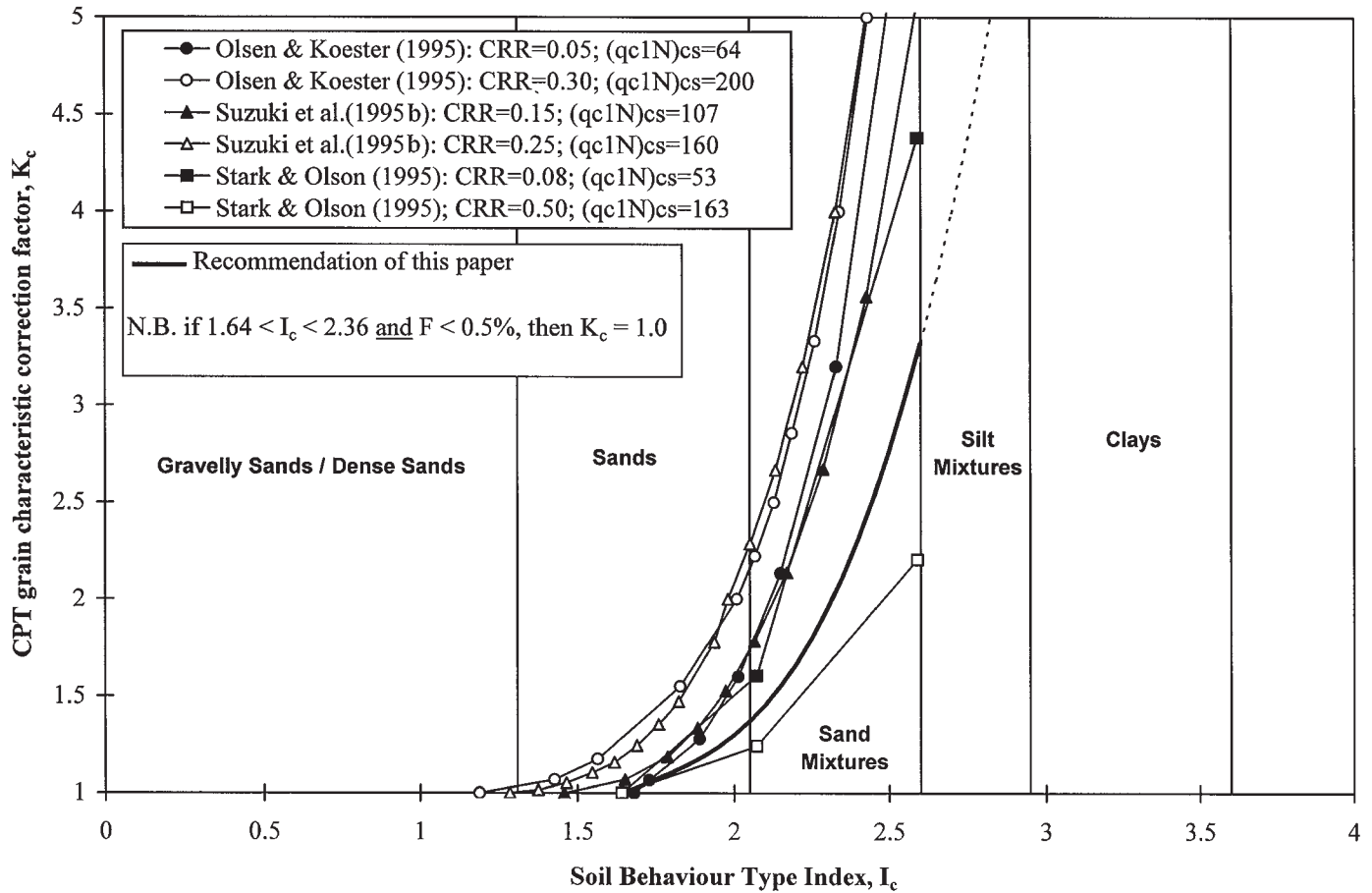
Fig. 15. Approximate comparison of various methods for correcting CPT tip resistance to clean sand equivalent values, based on soil behaviour type.
