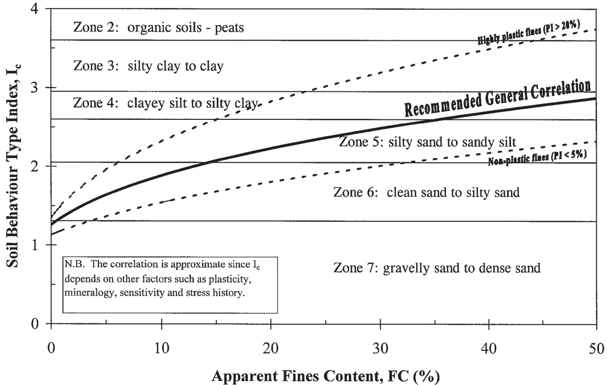
Fig. 9. Variation of CPT soil behaviour type index ( I_c ) with apparent fines content in or close to the normally consolidated zone of the soil behaviour chart by Robertson (1990). PI, plasticity index.
