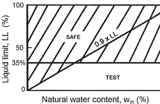
Fig. 4. Graphical representation of liquefaction criteria for silts and clays from studies by Seed et al. (1973) and Wang (1979) in China (after Marcuson et al. 1990): < 15\% finer than 0.005 mm, liquid limit (LL) < 35\% , and water content > 0.9 \times liquid limit.
