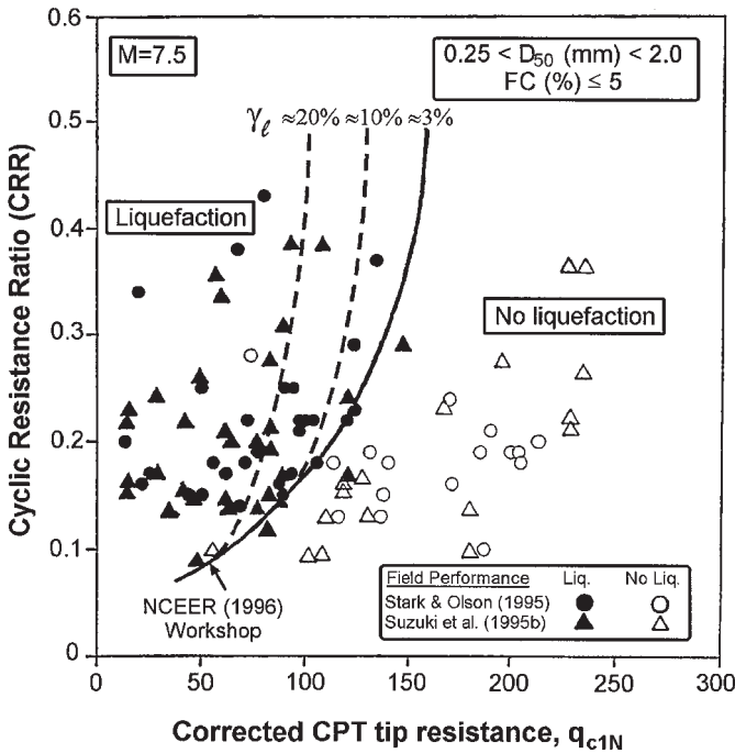
Fig. 6. Recommended cyclic resistance ratio (CRR) for clean sands under level ground conditions based on CPT. \gamma_l , limiting shear strain.
