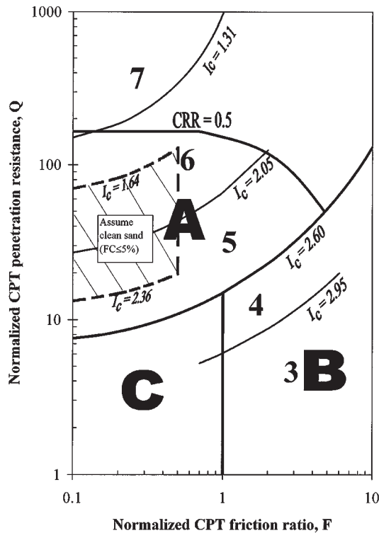
Fig. 16. Summary of liquefaction potential on soil classification chart by Robertson (1990). Zone A, cyclic liquefaction possible, depending on size and duration of cyclic loading; zone B, liquefaction unlikely, check other criteria; zone C, flow liquefaction and (or) cyclic liquefaction possible, depending on soil plasticity and sensitivity as well as size and duration of cyclic loading.
