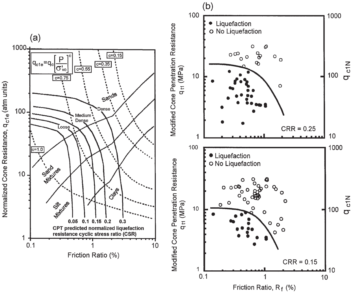
Fig. 14. Comparison of estimating CRR from the CPT. (a) CRR = 0.05 to 0.3, after Olsen and Koester (1995). c , stress exponent. (b) CRR = 0.15 and 0.25, after Suzuki et al. (1995b). \sigma'_v , vertical effective stress.
