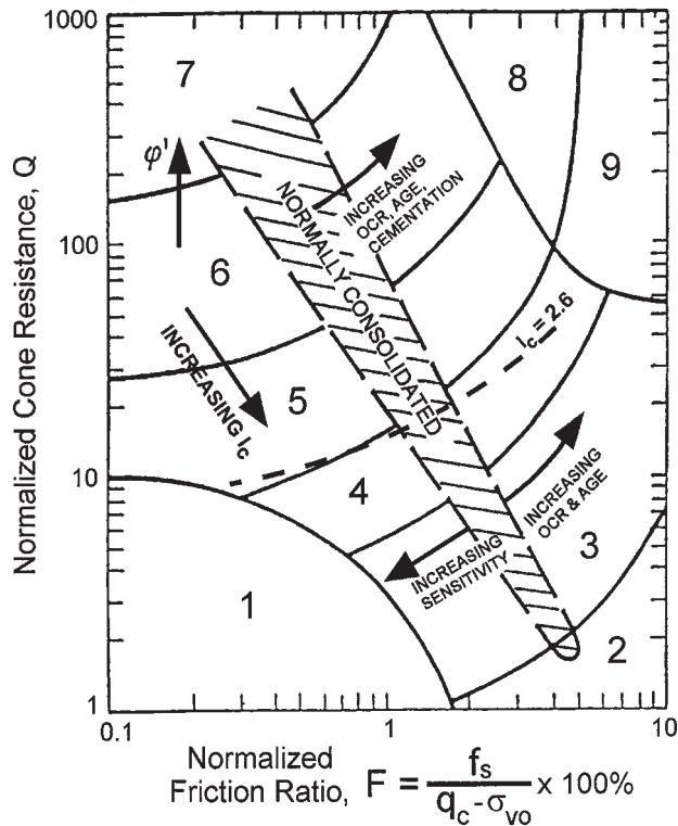
Fig. 8. Normalized CPT soil behaviour type chart, as proposed by Robertson (1990). Soil types: 1, sensitive, fine grained; 2, peats; 3, silty clay to clay; 4, clayey silt to silty clay; 5, silty sand to sandy silt; 6, clean sand to silty sand; 7, gravelly sand to dense sand; 8, very stiff sand to clayey sand (heavily overconsolidated or cemented); 9, very stiff, fine grained (heavily overconsolidated or cemented). OCR, overconsolidation ratio; \phi' , friction angle.
