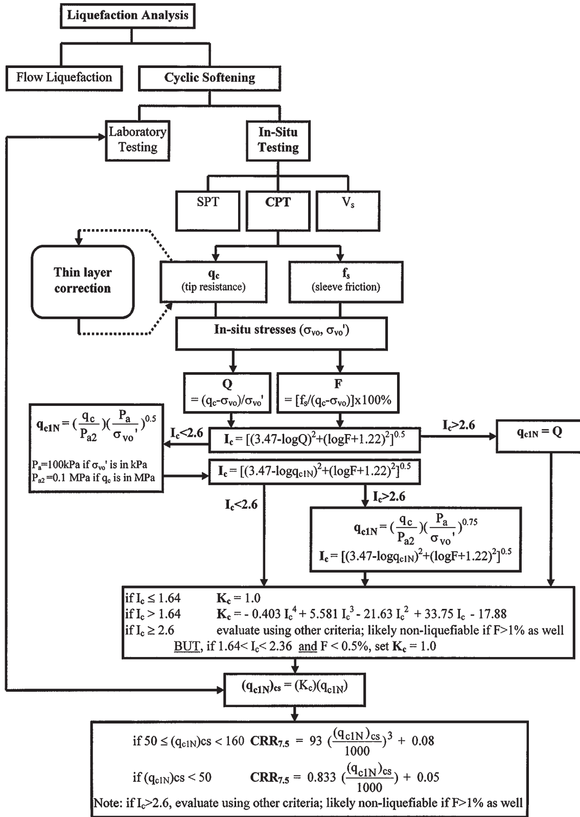
Fig. 12. Flow chart illustrating the application of the integrated CPT method of evaluating cyclic resistance ratio (CRR) in sandy soils. V_s , shear wave velocity.
