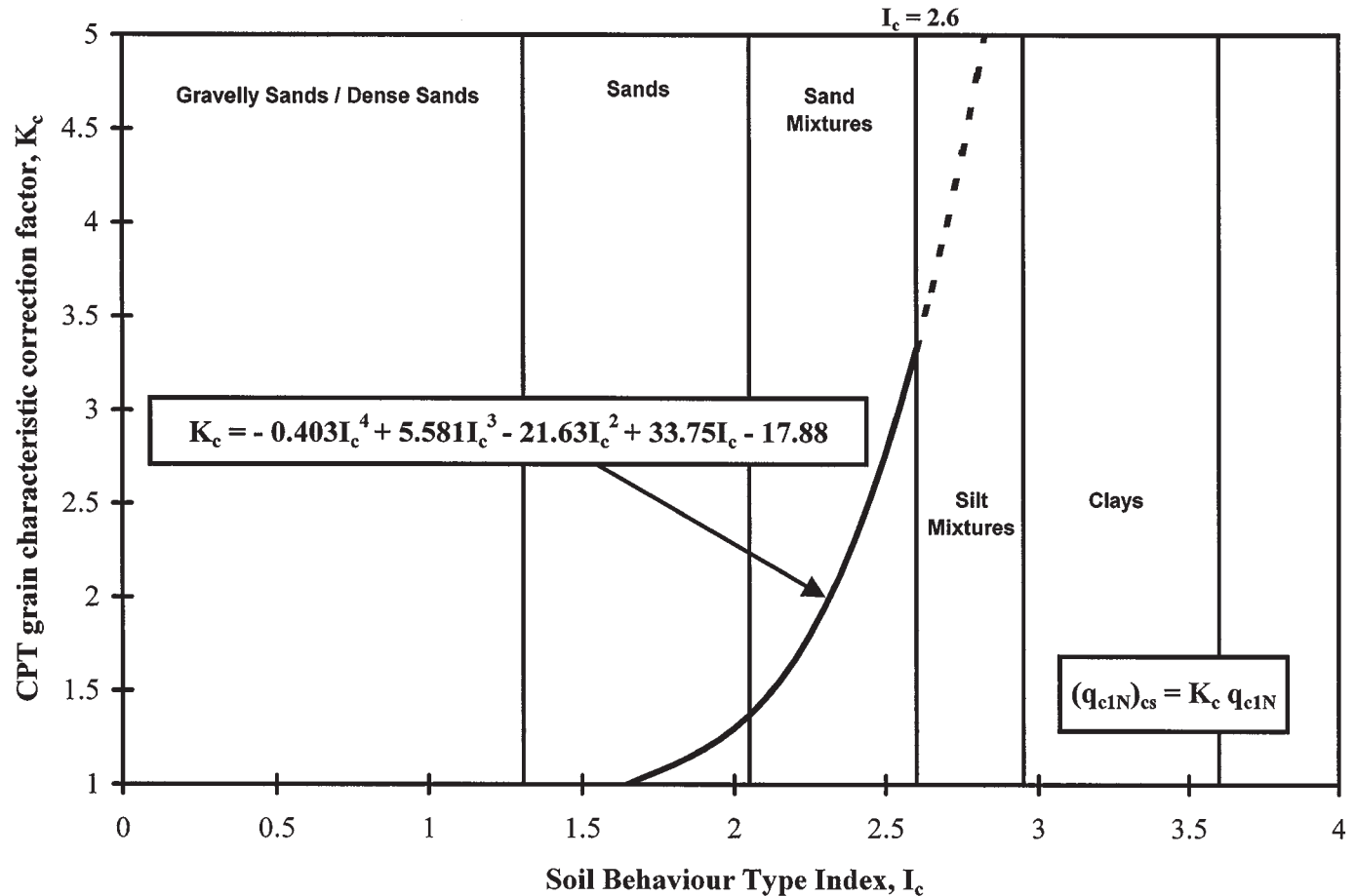
Fig. 10. Recommended grain characteristic correction to obtain clean sand equivalent CPT penetration resistance in sandy soils.
