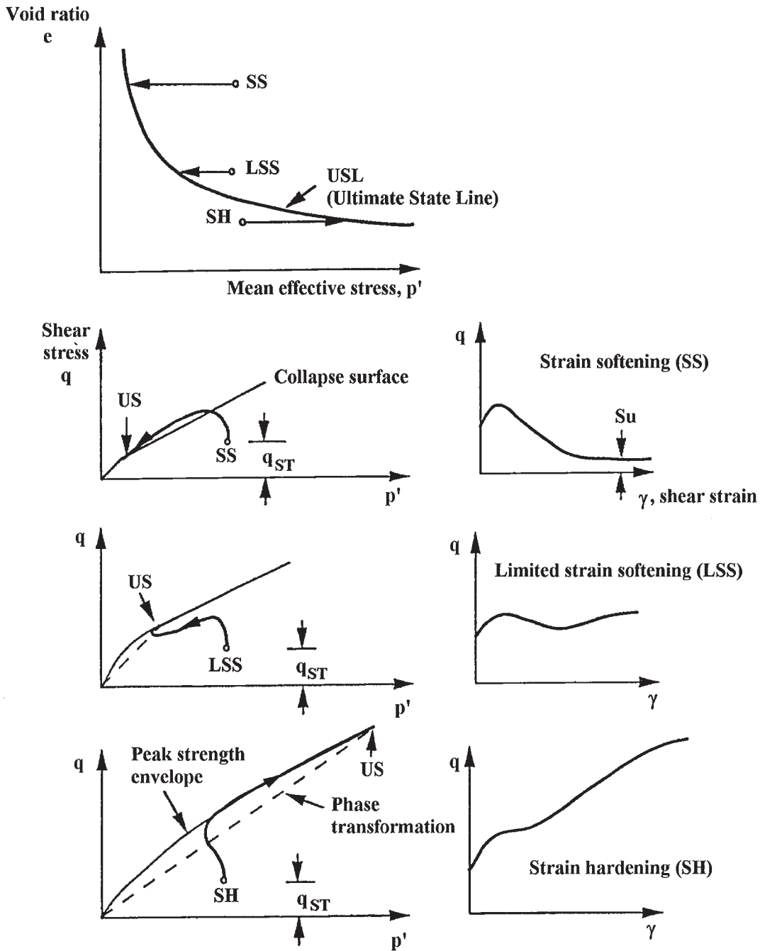
Fig. 1. Schematic of undrained monotonic behaviour of sand in triaxial compression (after Robertson 1994). LSS, limited strain-softening response; q_{ST} , static gravitational shear stress; S_u , ultimate undrained shear strength; SH, strain-hardening response; SS, strain-softening response; US, ultimate state.
