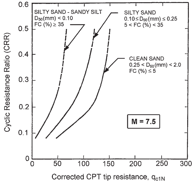
Fig. 7. Summary of variation of cyclic resistance ratio (CRR) with fines content based on CPT field performance data (after Stark and Olson 1995).
