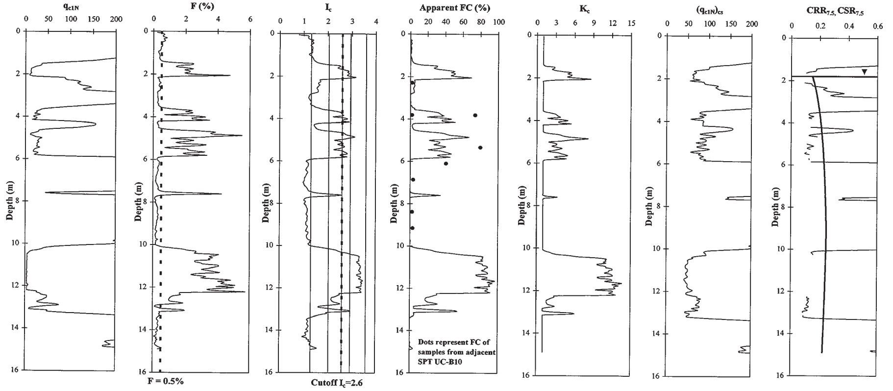
Fig. 13. Application of the integrated CPT method for estimating cyclic resistance ratio (CRR) to the State Beach site at Moss Landing which suffered cyclic liquefaction during the 1989 Loma Prieta earthquake in California.
