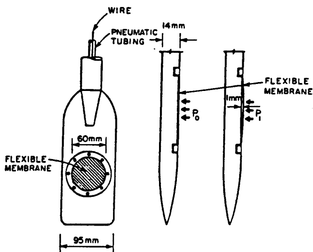
FIG. 1—Marchetti flat plate dilatometer.
