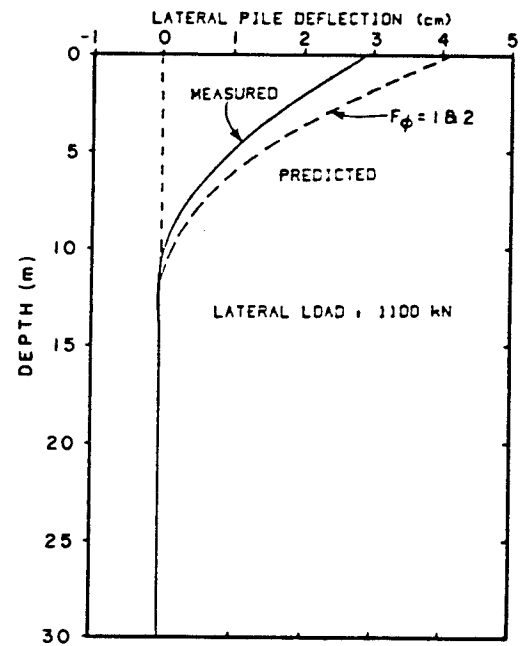
FIG. 7—Predicted versus measured lateral pile behavior: MOTH test pile.
