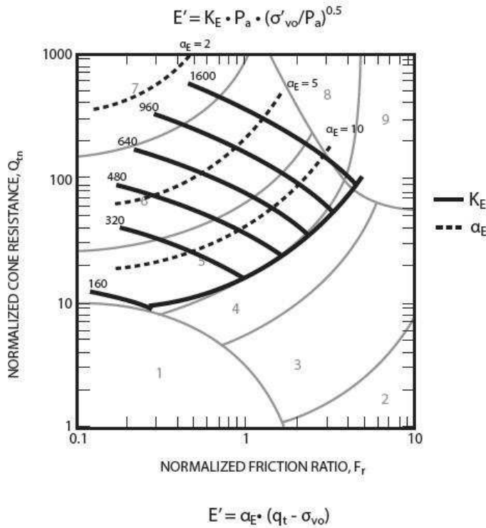
Figure 10: Contours of Young's modulus number, K_E (thick solid lines) and modulus factor \alpha_E , on normalized SBTn Q_{tm} - F_r chart for uncemented Holocene- and Pleistocene-age sandy soils (after Robertson, 2009a)
