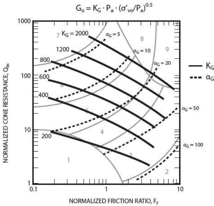
Figure 9: Contours of small strain modulus number, K_G (thick solid lines) and modulus factor \alpha_G , on normalized SBTn Q_{tm} - F_r chart for uncemented Holocene- and Pleistocene-age sandy soils (After Robertson, 2009a)
