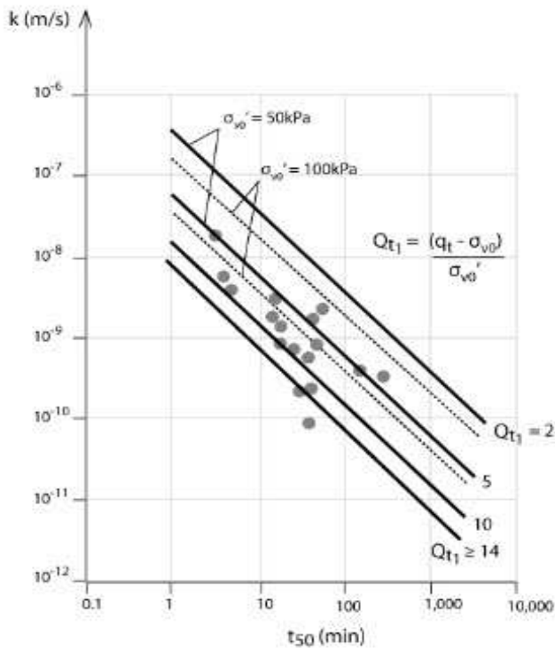
Figure 12: Relationship between CPTu t_{50} (in minutes) and soil permeability ( k ) and normalized cone resistance, Q_{t1} (data from Robertson et al, 1992)
